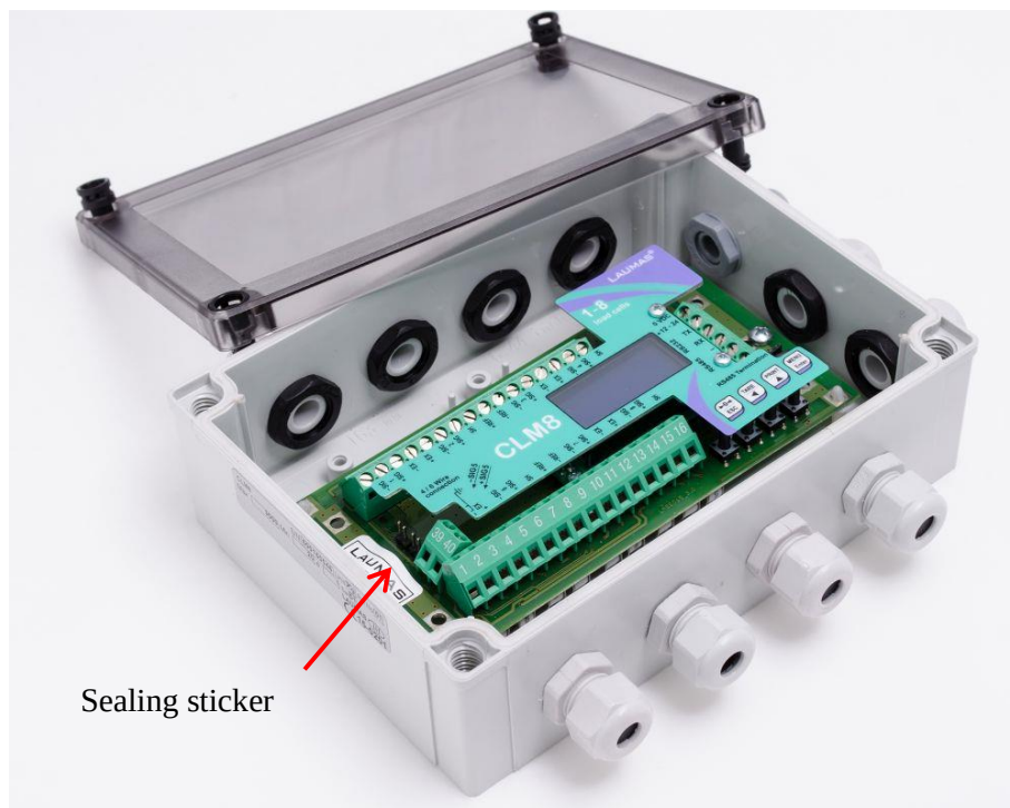
Figure 4 CLM8 indicator – sub model CLM8PC
