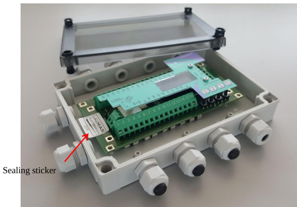
Figure 5 CLM8 indicator – sub model CLM8PCN
