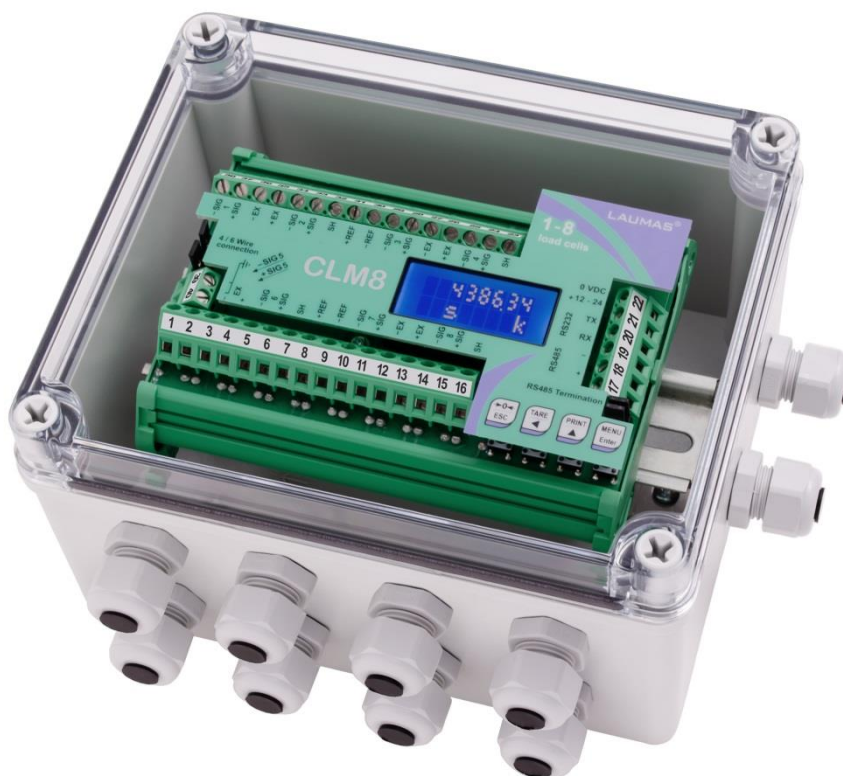
Figure 2 CLM8 indicator – sub model CLM8CASTL
