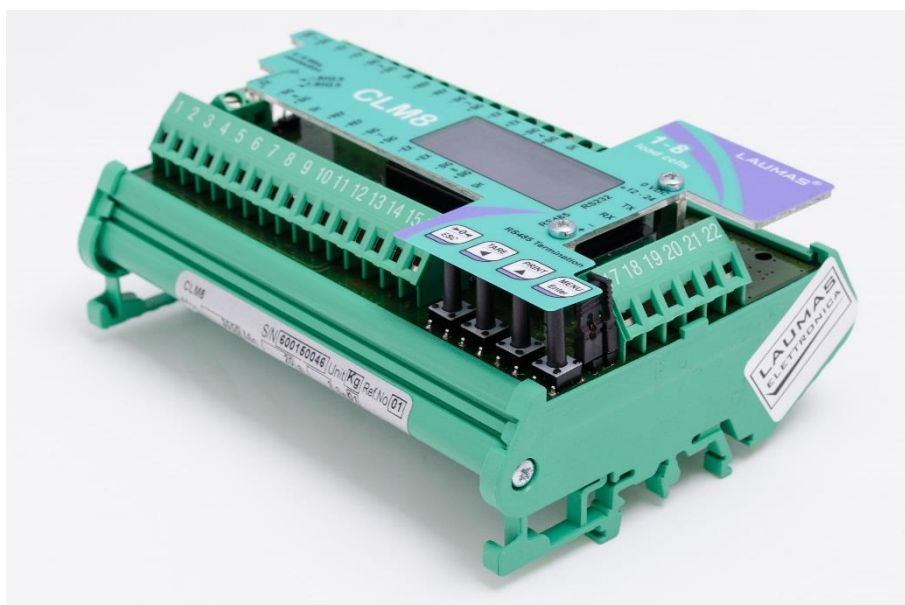
Figure 8 Sealing of CLM8 indicator – for DIN rail mounting.
