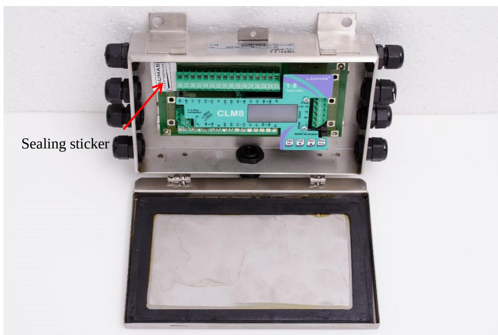
Figure 7 CLM8 indicator – sub model CLM8INOX, sealed.
